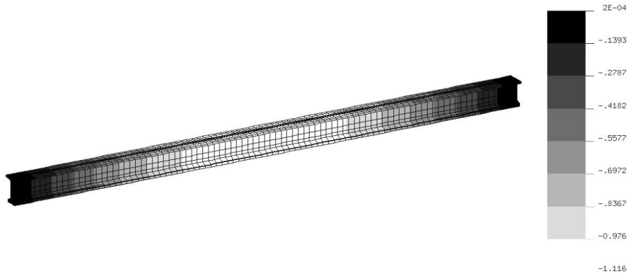
Figure 13. Downward deflection due to the self-weight of the girder, computed using first-order elastic finite element analysis
