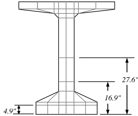
Figure 11. Computer model of the cross section of the girder neglecting prestressed steel
