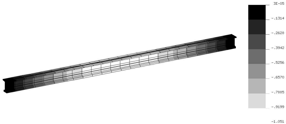
Figure 20. Downward deflection of the girder (with its cross section property accounting for prestressed steel) due to the self-weight of the girder
