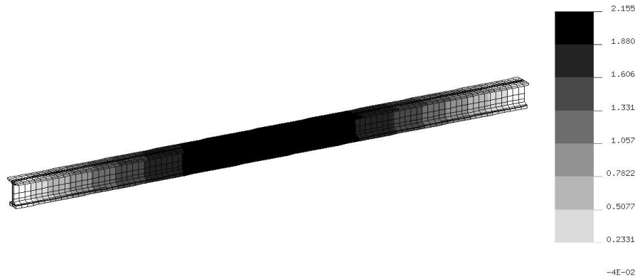
Figure 15. Camber due to equivalent loads (produced by prestressed steel) in combination with the self-weight of the girder, computed using first-order elastic finite element analysis
