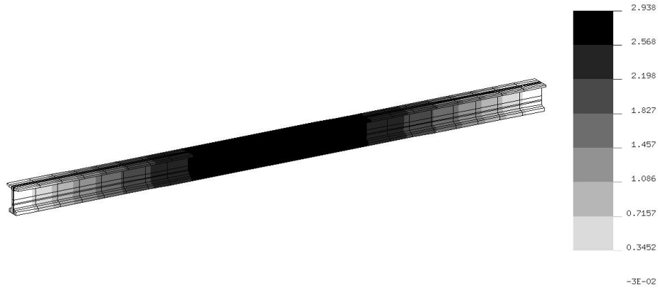
Figure 21. Camber of the girder (with its cross section property accounting for prestressed steel) computed using the thermal effects method
