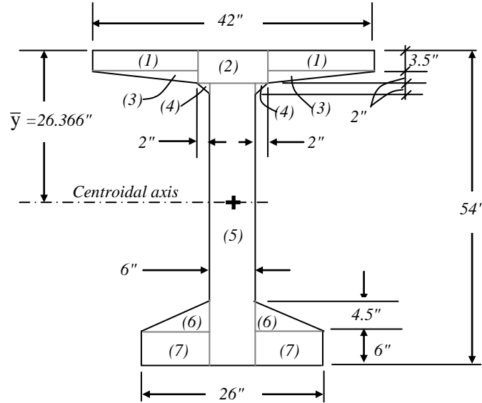
Figure 6. Gross section of the I-girder for the camber computation example
