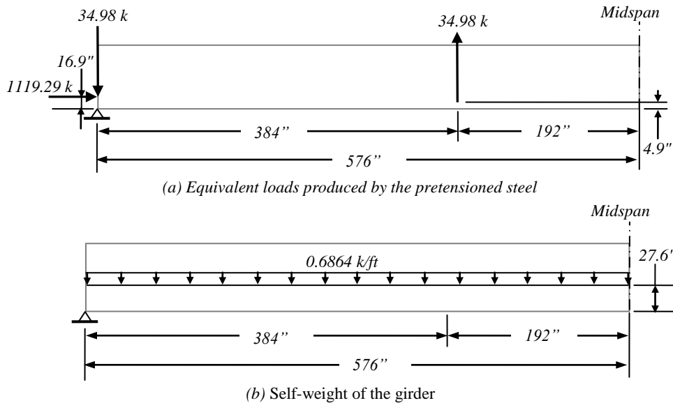
Figure 10. Equivalent loads (produced by prestensioned steel) and the self-weight of the girder
